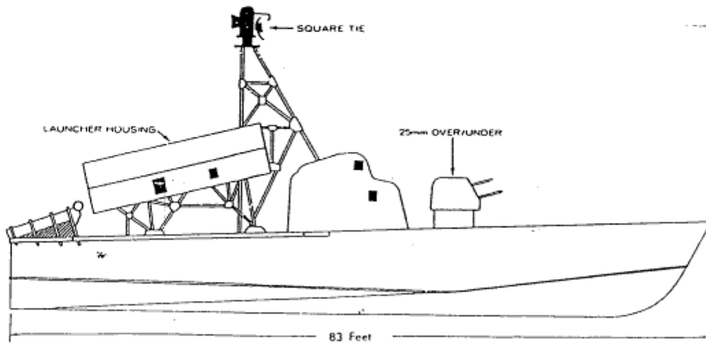
USSR 'KOMAR' CLASS PG
