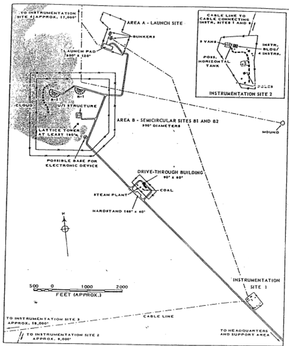
MISSILE LAUNCH COMPLEX B, SARY SHAGAN
