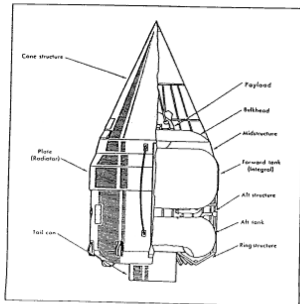
LUNIK UPPER STAGE
